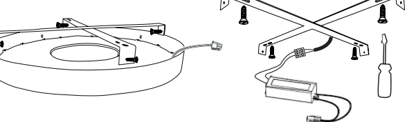
Surface mounted luminaire
